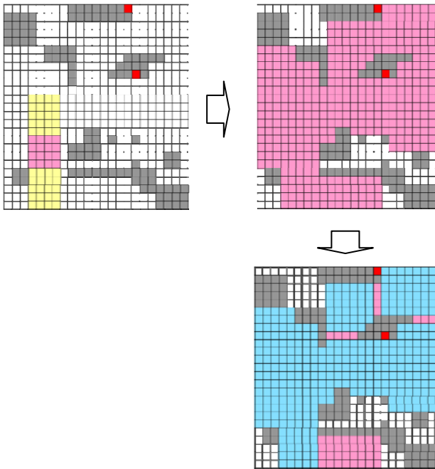
Figure 5: Recursive fill algorithm to find accessible space
