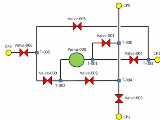
Figure 8: PID of 7 valves
