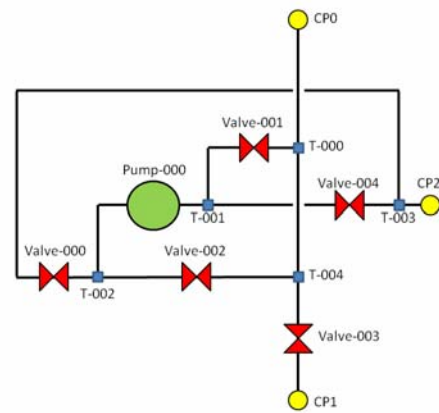
Figure 7: PID of 5 valves
