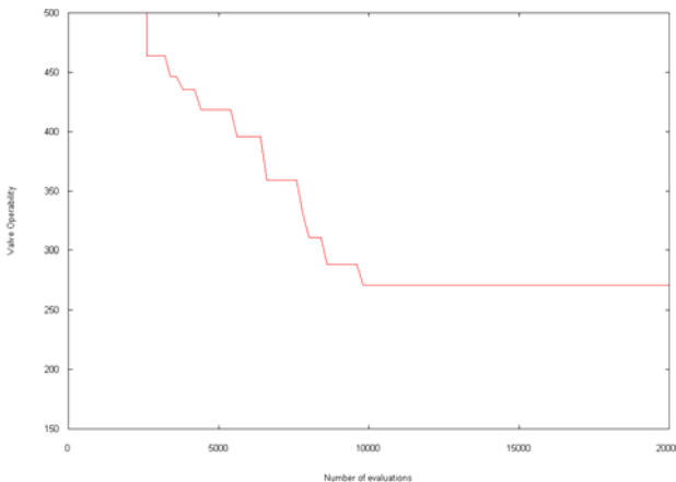
Figure 14: Best solution of valve operability in GA population
