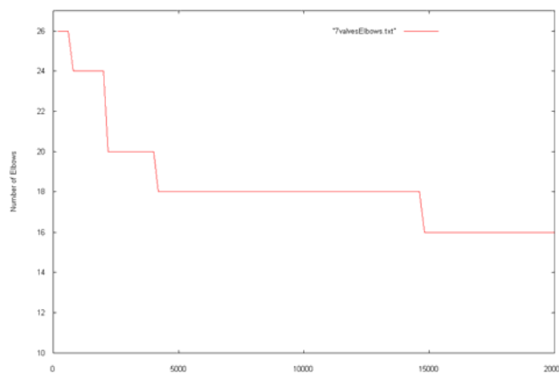
Figure 13: Best solution of number of elbows in GA population
