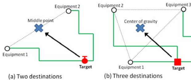
Figure 3: A basic concept of the self-organization
