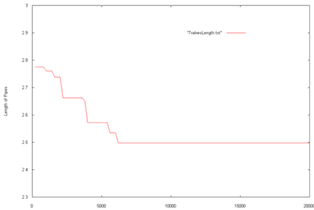
Figure 12: Best solution of material cost in GA population
